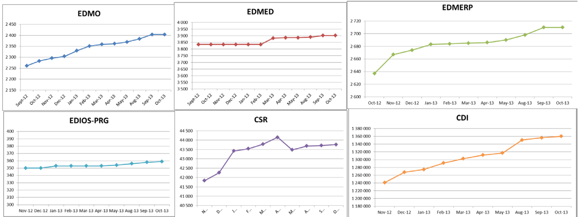
Figure 1 - Global counts on all catalogues
